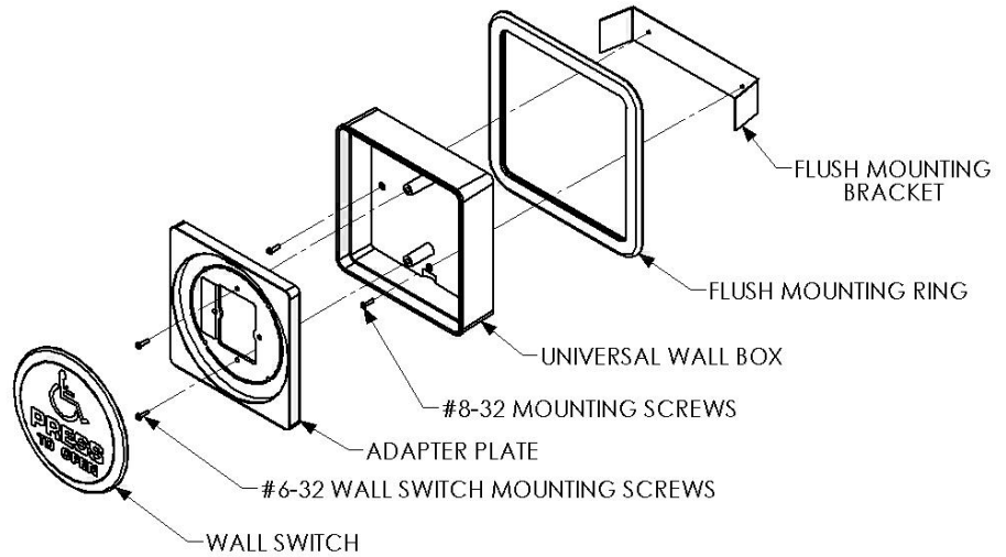
FLUSH MOUNT KIT ASSEMBLY INSTRUCTIONS
