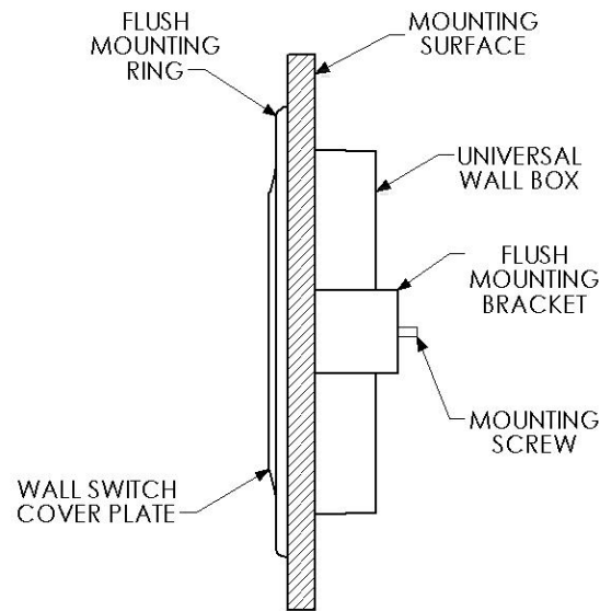
FLUSH MOUNTING ILLUSTRATION
