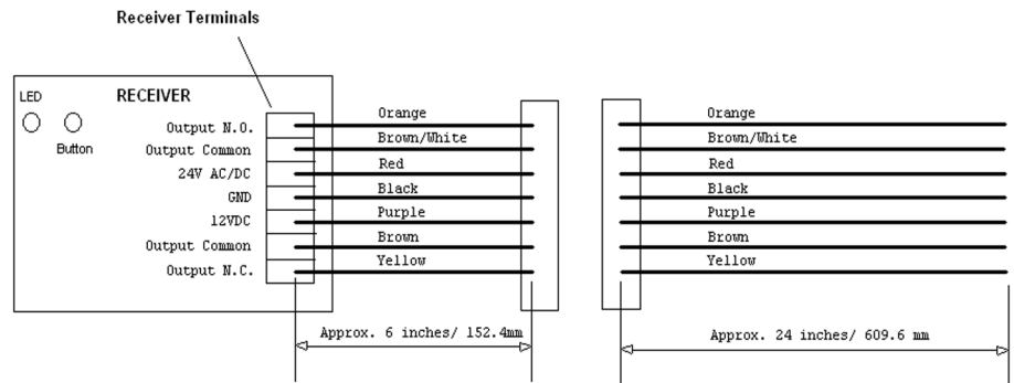
Diagram 2: Receiver Wiring Harness.
